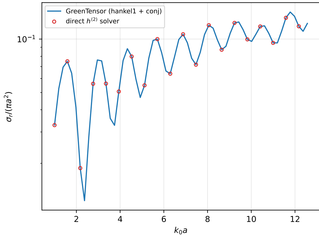
Backscatter of the 8-layer Fuchs LL: identical observables
