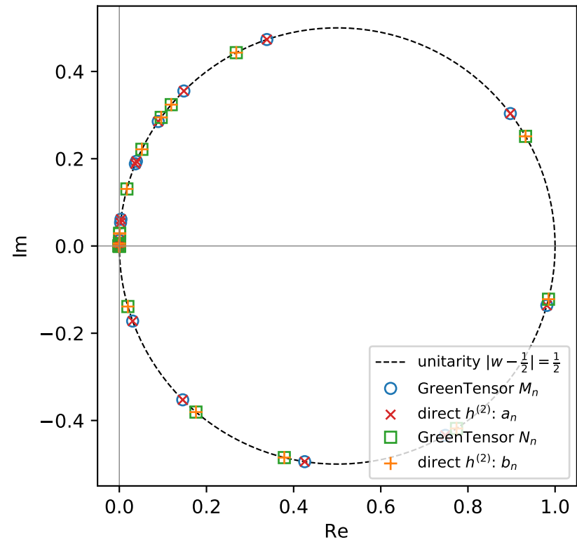
8-layer Fuchs LL, k_0 a = 4\pi : M_n, N_n in e^{+j\omega t} canon
